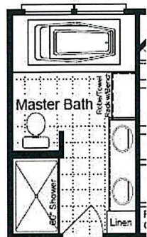
Optional Stand Alone Tub & 60" Shower
